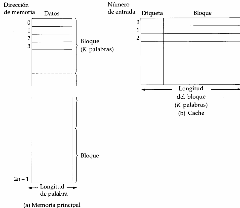
(a) Memoria principal FIGURA 1.19 Estructura de cache/memoria principal
