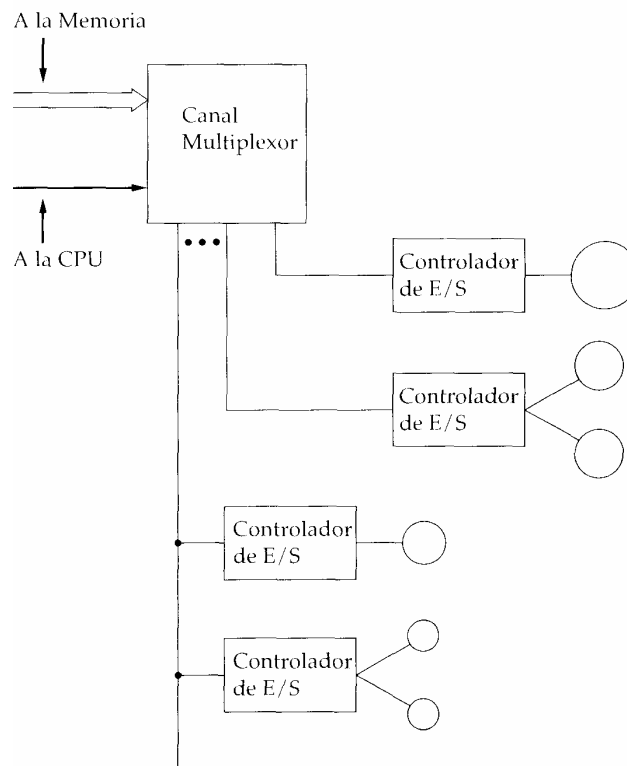
(b) Multiplexor
