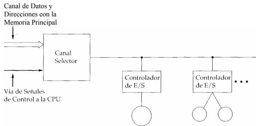
(a) Selector
